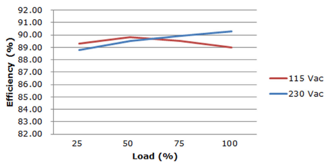
VOF-85B-24 Efficiency vs. Output Load (Natural Convection)
