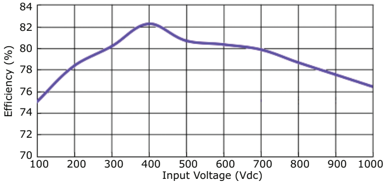
AE15-EW-S15 Efficiency Curve Efficiency vs. Input Voltage
