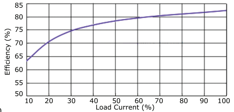
AE15-EW-S24-T Efficiency Curve Efficiency vs. Load Current
