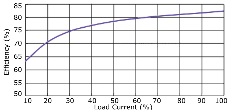
AE15-EW-S24-DIN Efficiency Curve Efficiency vs. Load Current
