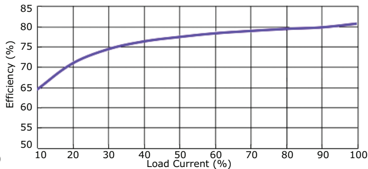
AE15-EW-S15-DIN Efficiency Curve Efficiency vs. Load Current
