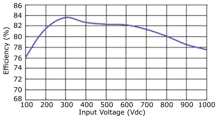
AE15-EW-S24-DIN Efficiency Curve Efficiency vs. Input Voltage
